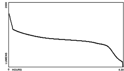
XPR-5582 PERFORMANCE CURVE
